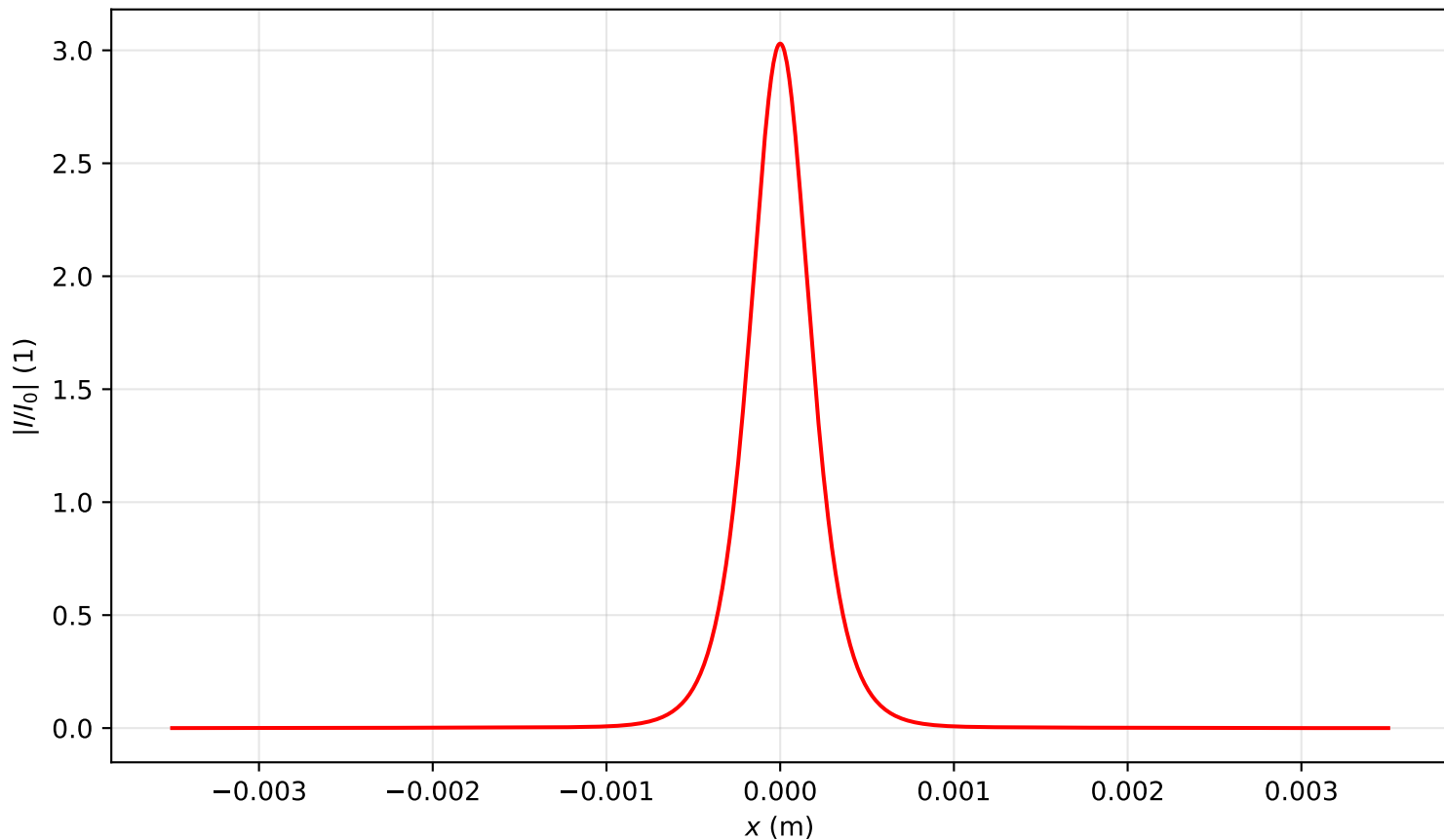
Intensity profile I(x, y = 0, z = 3.582)/I_0 , P_{in}=1.0P_{cr} , artificial time
